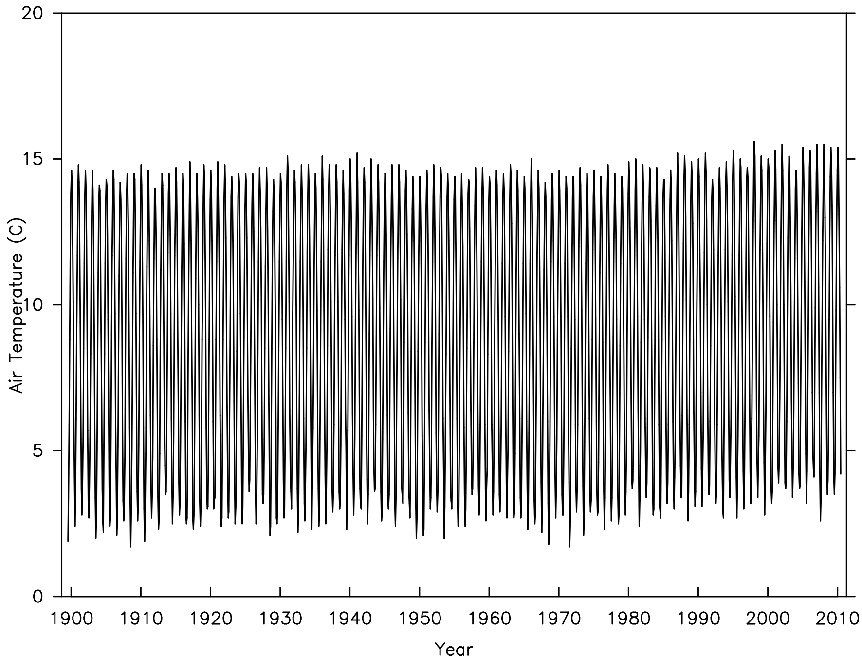
Land-Surface-Average Monthly Mean Air Temperature 1900-2010
