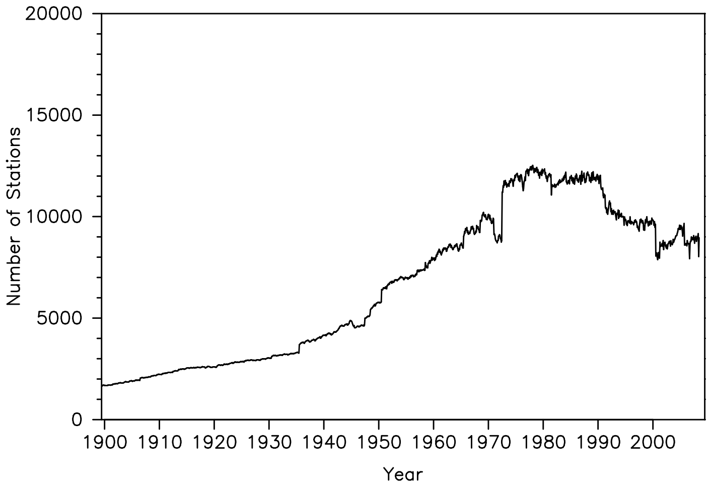
Number of Air Temperature Stations 1900 – 2008
